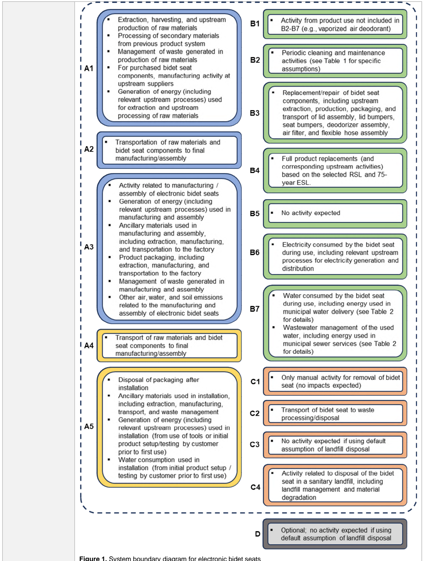
Figure 1. System boundary diagram for electronic bidet seats
